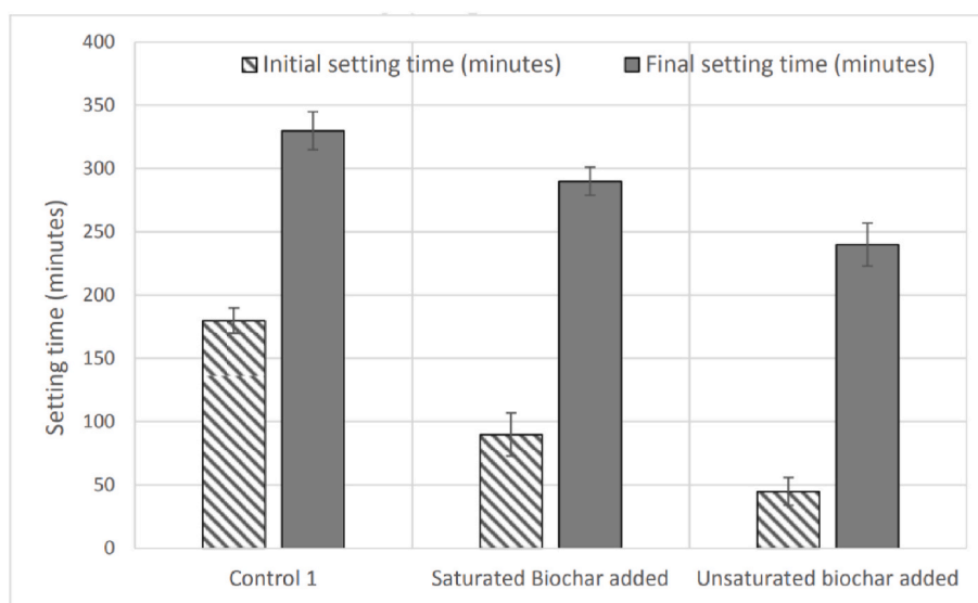
Fig. 2. Initial and final setting times based on the addition of \text{CO}_2 adsorbed and non- \text{CO}_2 adsorbed biochar [89].
