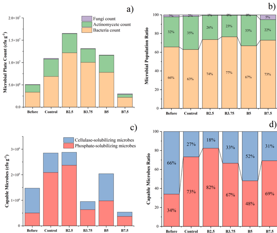
Fig. 10. The results of microbial population (a), Microbial population ratio (b), Capable microbes (c) and Capable microbes ratio (d), under different coffee pulp biochar application rates.
