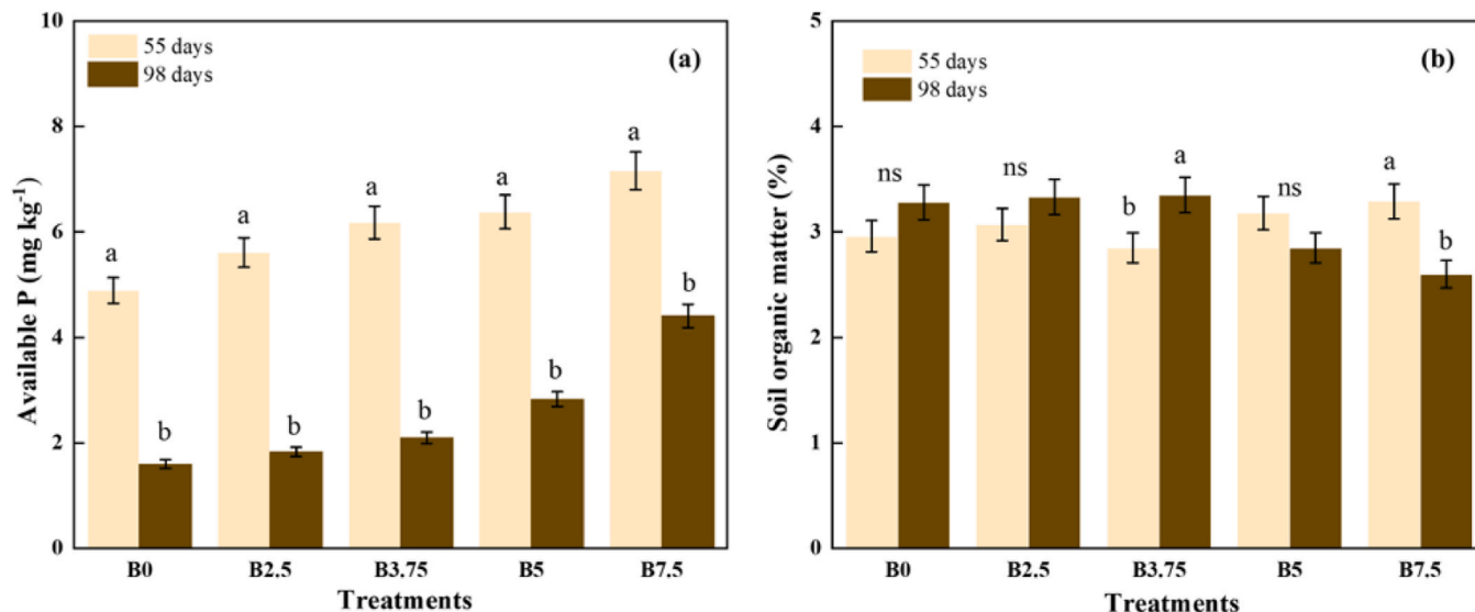
Fig. 6. Soil available P (a) and soil organic matter (b) after treated with different dosages of coffee pulp biochar. Distinct letters indicate statistically significant differences ( p < 0.05 ).
