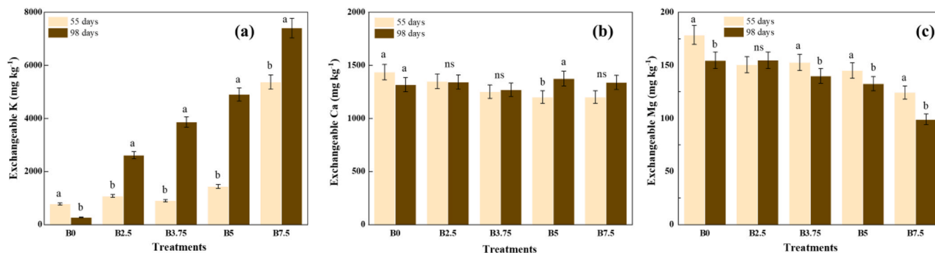
Fig. 7. Soil exchangeable K (a), exchangeable Ca (b), and exchangeable Mg (c) after treated with different dosages of coffee pulp biochar. Distinct letters indicate statistically significant differences ( p < 0.05 ).
