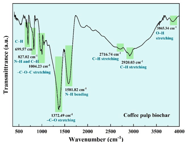
Fig. 5. Fourier transforms infrared spectroscopy (FTIR) spectra of coffee pulp biochar.
