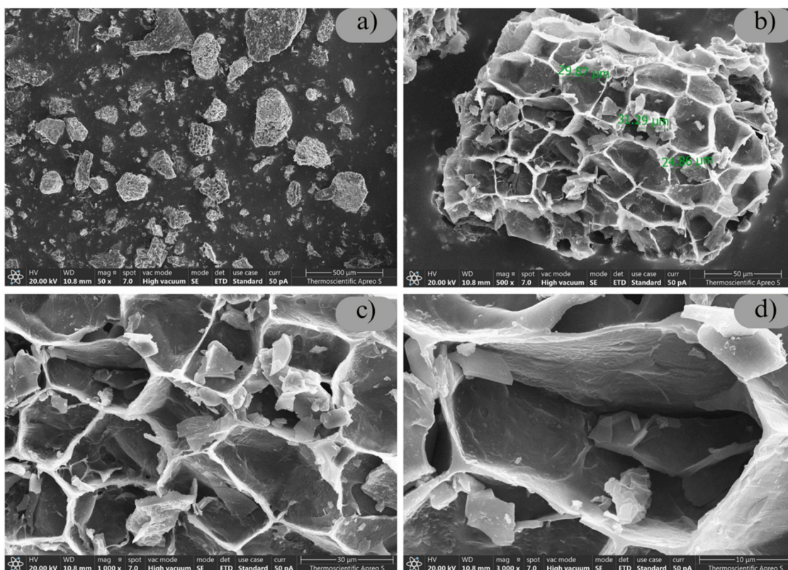
Fig. 3. Surface morphology of synthesized coffee pulp biochar at different magnifications of 50 × (a), 500 × (b), 1000 × (c) and 3000 × (d).
