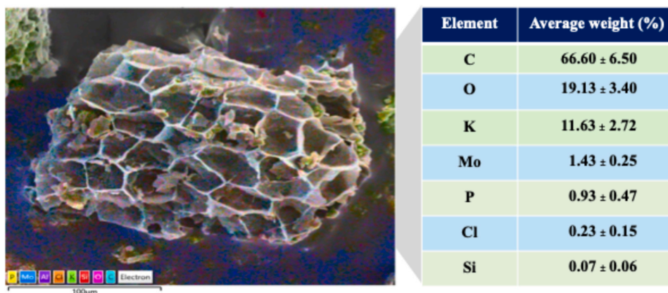
Fig. 4. Elemental components of coffee pulp biochar.
