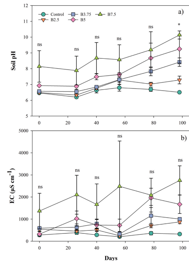
Fig. 8. Soil pH (a) and soil EC (b) after incubation with different dosage of coffee pulp biochar. Note: * = Significant difference at p < 0.05 , ns = Non-statistical significant difference at p < 0.05 . Error bars = Standard Error.
