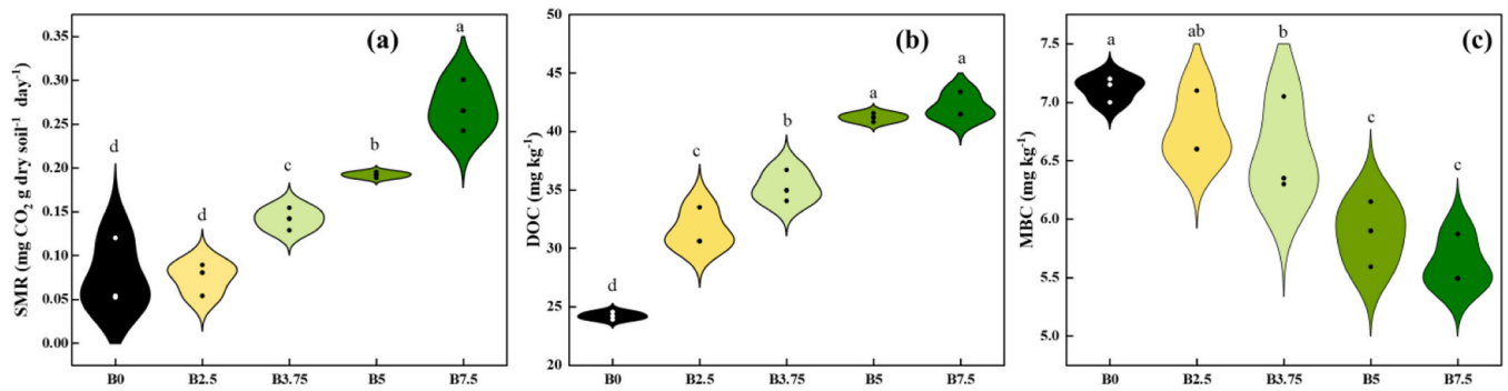
Fig. 9. Levels of Soil Microbial Respiration (SMR) (a), Dissolved Organic Carbon (DOC) (b), and Microbial biomass carbon (MBC) (c) under treated with coffee pulp biochar for 98 days. Distinct letters indicate statistically significant differences ( p < 0.05 ).
