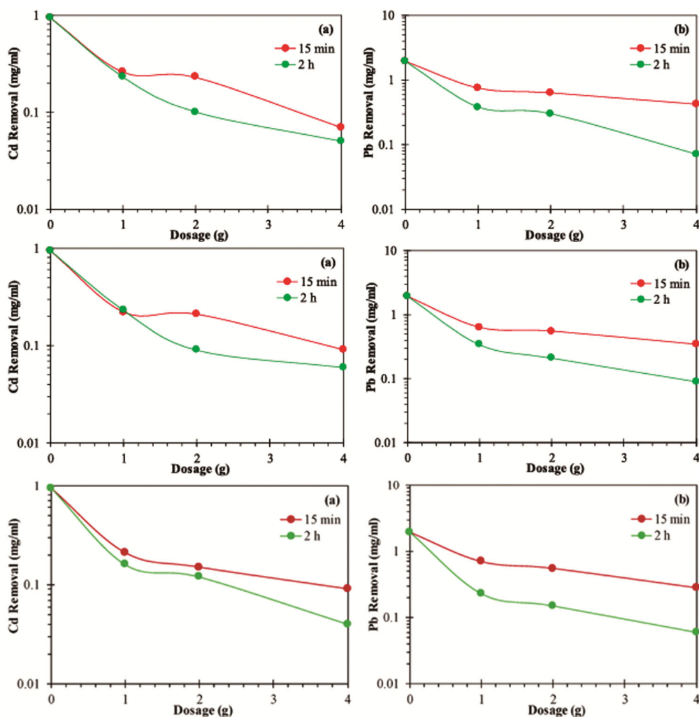
Fig. 6 — Heavy metal removal performance by biochar derived from corncob, rice husk and wheat straw (a) cadmium removal and (b) lead removal (source: 28 )
