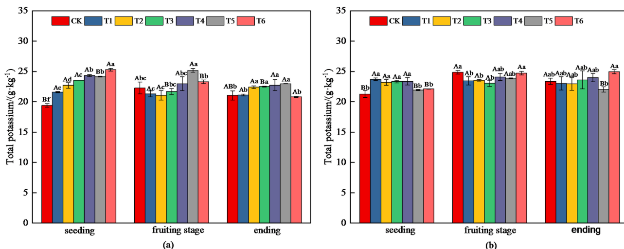
Fig. 4. During the whole growth period, different treatments of 0–20 cm (a) and 20–40 cm (b) soil layer total potassium.
