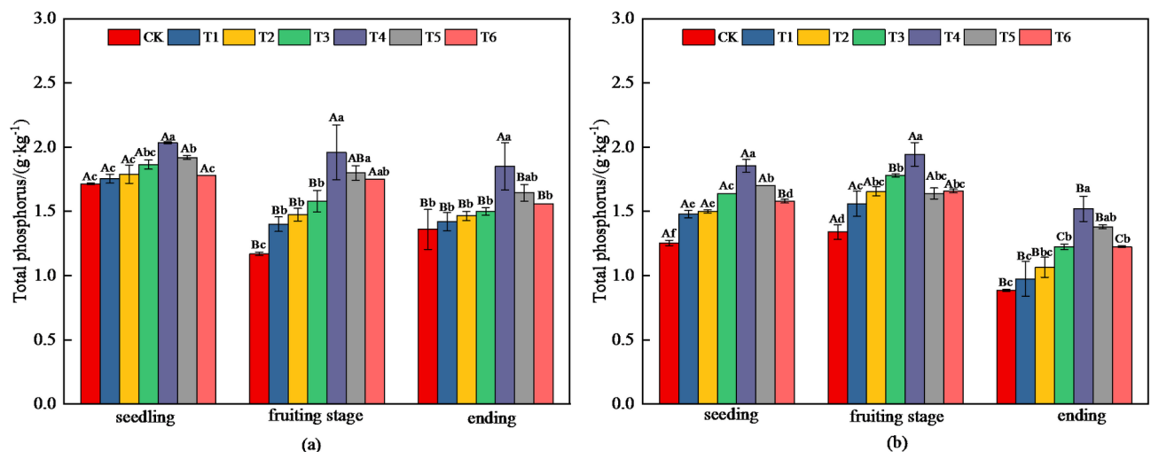
Fig. 3. During the whole growth period, different treatments of 0–20 cm (a) and 20–40 cm (b) soil layer total phosphorus.
