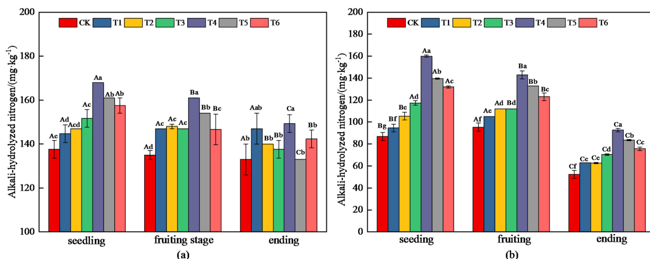
Fig. 6. During the whole growth period, different treatments of 0–20 cm (a) and 20–40 cm (b) soil layer alkali-hydrolyzed nitrogen.
