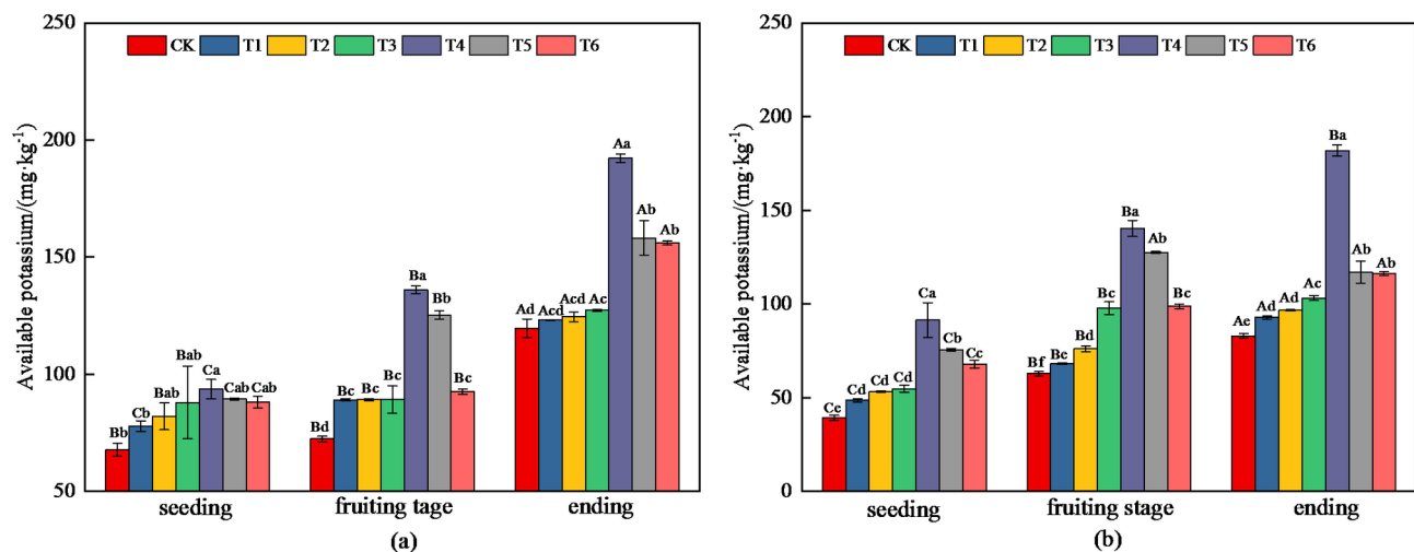
Fig. 8. Available potassium of tomato in 0–20 cm (a) and 20–40 cm (b) soil layers under different treatments during the whole growth period.
