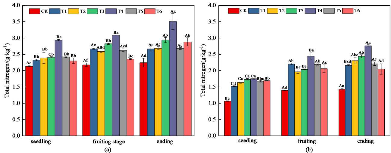
Fig. 2. During the whole growth period, different treatments of 0–20 cm (a) and 20–40 cm (b) soil layer total nitrogen.
