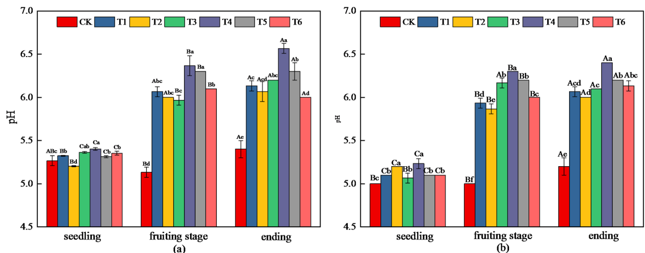
Fig. 1. The characteristics of pH changes in 0–20 cm (a) and 20–40 cm (b) soil layers under different treatments during the whole growth period of tomato. Note: Different lowercase letters indicate significant difference of the same soil layer in the same period among different treatments, while different uppercase letters indicate significant difference of the same soil layer between same treatments in the different period ( P < 0.05 ), the same below.
