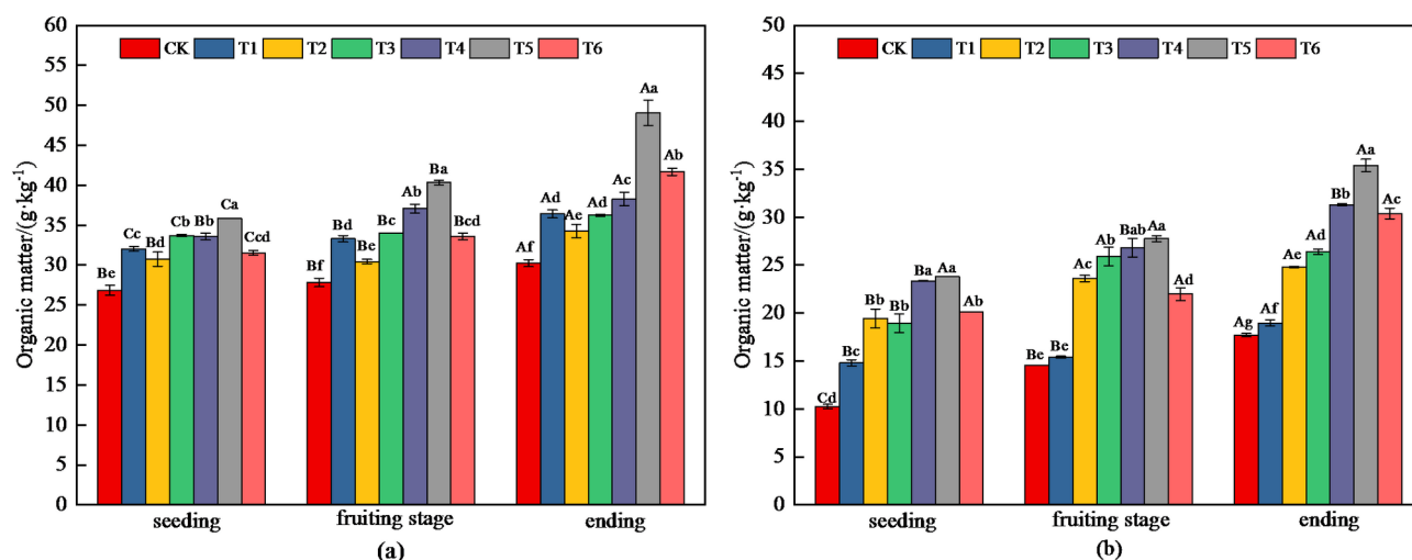
Fig. 5. Different treatments of organic matter in 0–20 cm (a) and 20–40 cm (b) soil layers during the whole growth period of tomato.
