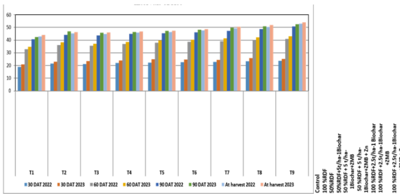
Fig. 4. Effect of biochar and fertility levels on root volume at different intervals of rice
