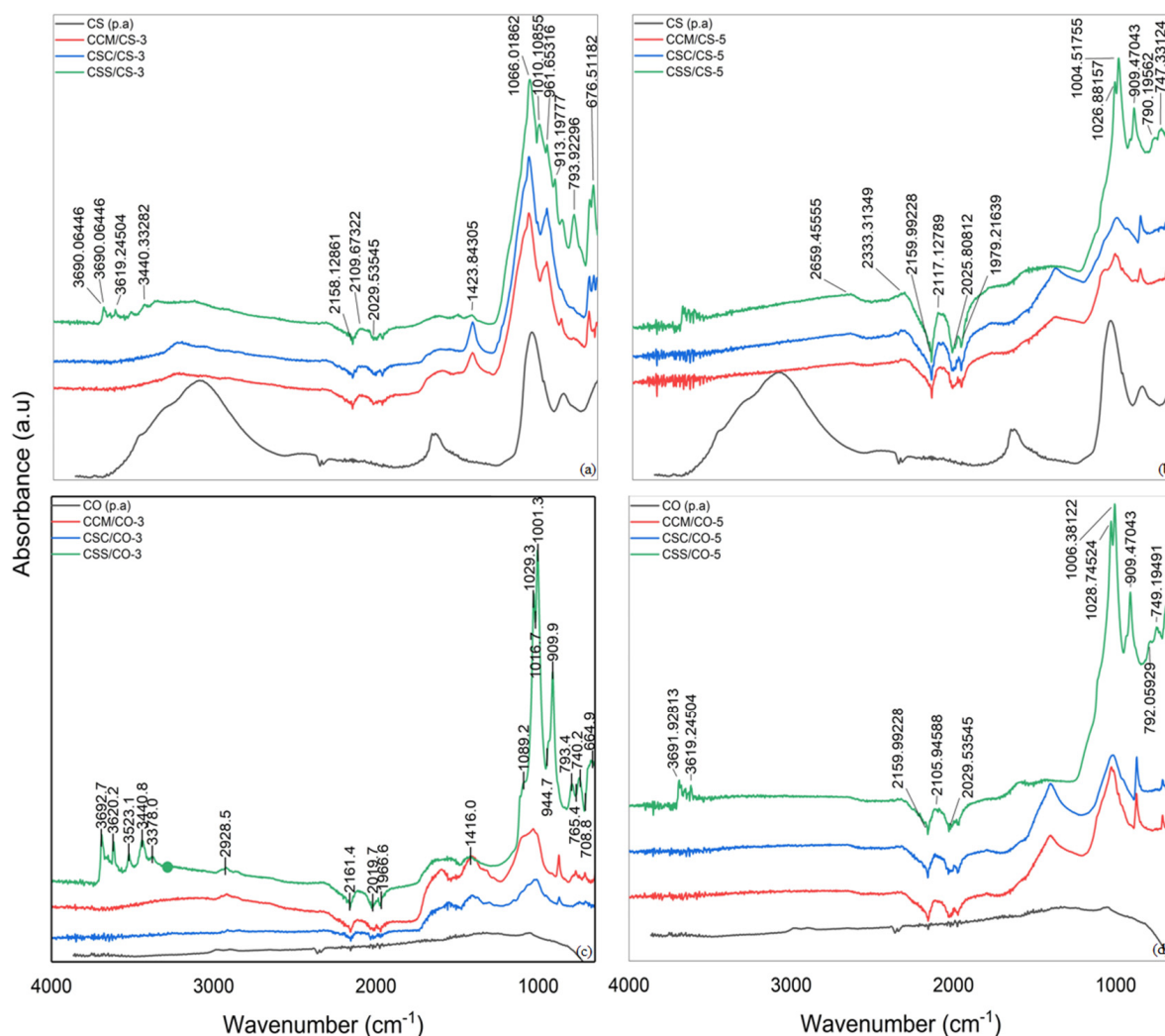
Figure 2. Fourier transform infrared spectroscopy with attenuated total reflection (ATR-FTIR) and the main peaks and characteristics of the chemical groups found in composites produced from biochar, doped or not with copper sulfate or copper oxide. (a) Composites doped with copper sulfate at 300 °C; (b) composites doped with copper sulfate at 550 °C; (c) composites doped with copper oxide at 300 °C and (d) composites doped with copper oxide at 550 °C.
