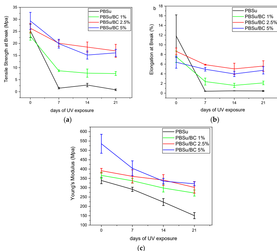
Figure 8. Variation in (a) tensile strength at break point, (b) elongation at break point, and (c) Young's Modulus of neat PBSu and its PBSu/BC composites during different days of UV exposure. Error bars represent standard deviation (SD) from three independent replicates (n = 3).
