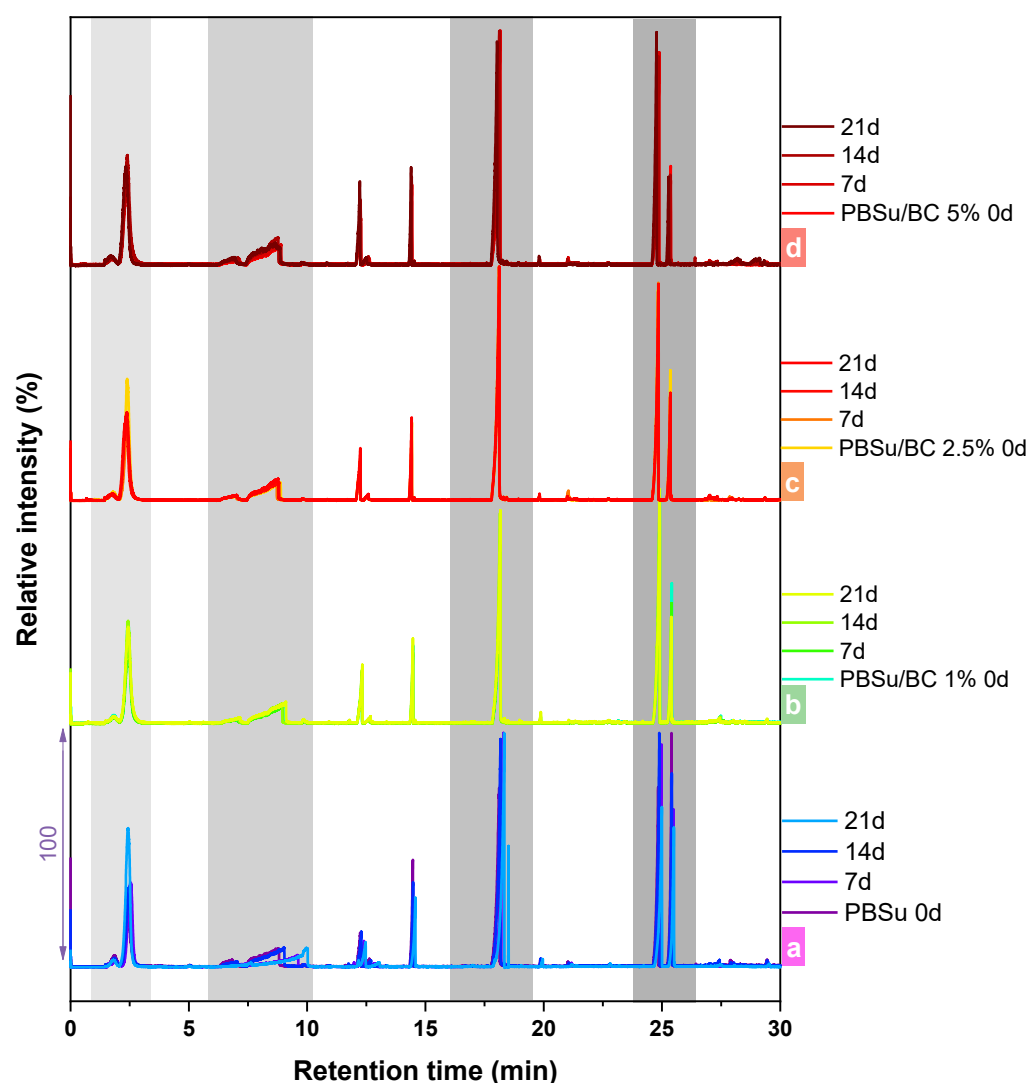
Figure 5. Total ion chromatograms (TICs) of (a) neat PBSu with different contents in biochar, (b) 1 wt.%, (c) 2.5 wt.%, and (d) 5 wt.%, during UV exposure testing for different intervals (7, 14, 21 days).
