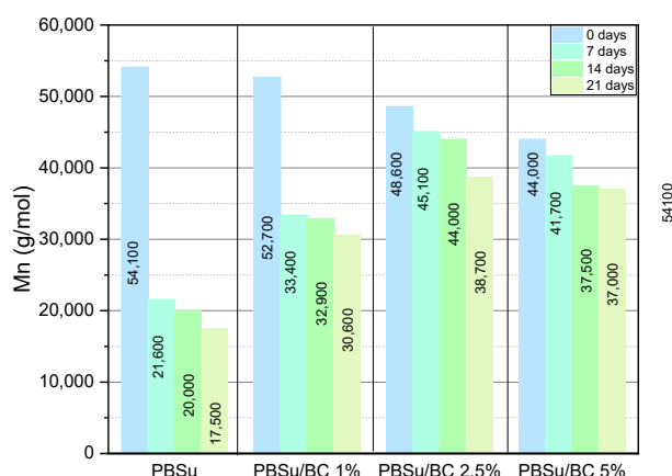
Figure 1. Molecular weight of PBSu and its composites during UV exposure.
