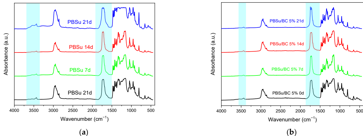
Figure 2. Stacked FT-IR spectra of (a) neat PBSu and (b) PBSu/BC 5 wt.% upon different UV radiation times.
