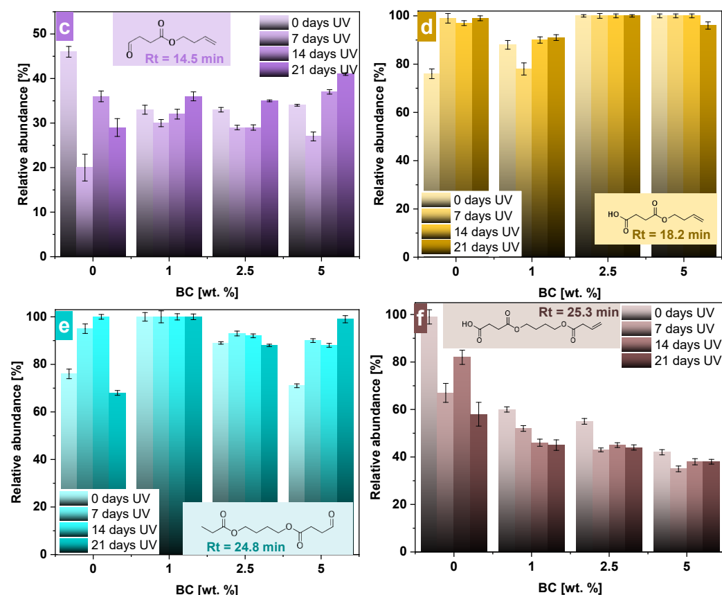
Figure 7. Profile of main decomposition products for different contents in BC in studied composites during UV exposure testing for 0, 1, 2, and 3 weeks. (a) Tetrahydrofuran; (b) succinic anhydride; (c) but-3-en-1-yl 4-oxobutanoate; (d) 4-(but-3-en-1-yloxy)-4-oxobutanoic acid; (e) 4-(propionyloxy)butyl 4-oxobutanoate; (f) 4-(4-(but-3-enoyloxy)butoxy)-4-oxobutanoic acid. Error bars represent standard deviation (SD) from three independent replicates (n = 3).
