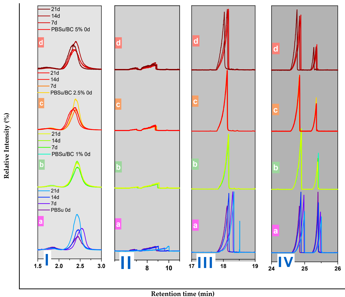
Figure 6. Enlarged TICs for (I) Rt = 1.5–3 min, (II) Rt = 6–11 min, (III) Rt = 17–19 min, and (IV) Rt = 24–26 min. As in Figure 5, the diagram's annotations are the following: (a) PBSu, (b) PBSu/BC 1 wt.%, (c) PBSu/BC 2.5 wt.%, and (d) PBSu/BC 5 wt.% for untreated samples and during UV testing.
