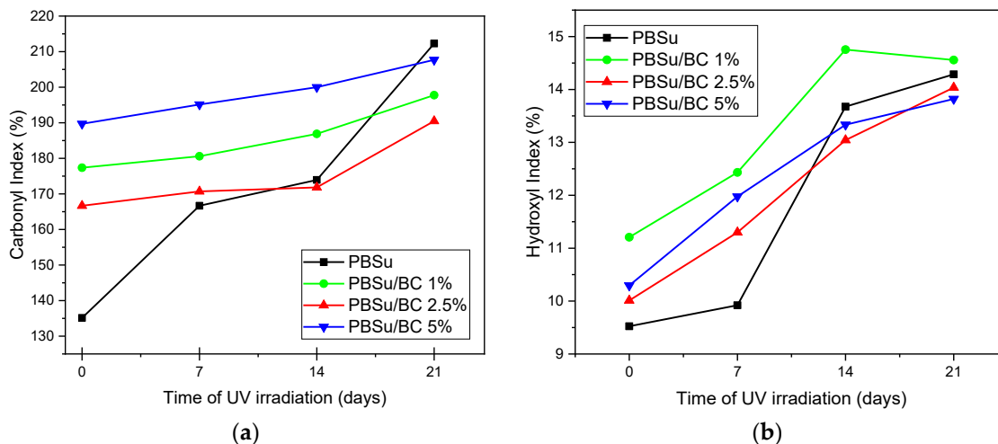
Figure 3. (a) Carbonyl index and (b) hydroxyl index of PBSu and its composites during UV exposure for 7, 14, and 21 days.
