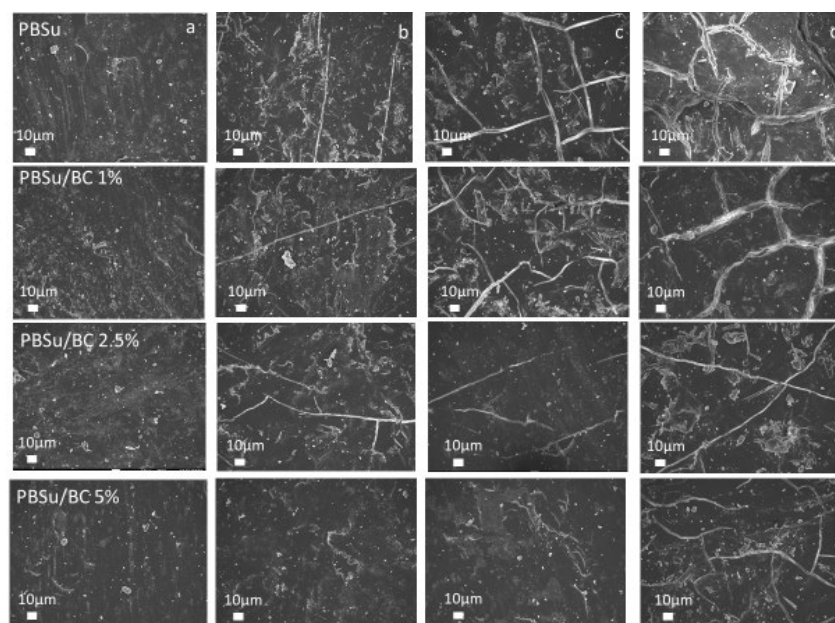
Figure 9. SEM micrographs of PBSu and its composites after (a) 0, (b) 7, (c) 14, and (d) 21 days of UV irradiation.
