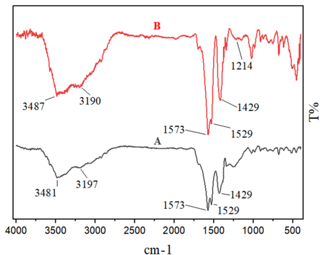
Figure 9. FT-IR spectra of Cu-L-histidine@biochar (A) and recovered Cu-L-histidine@biochar (B).
