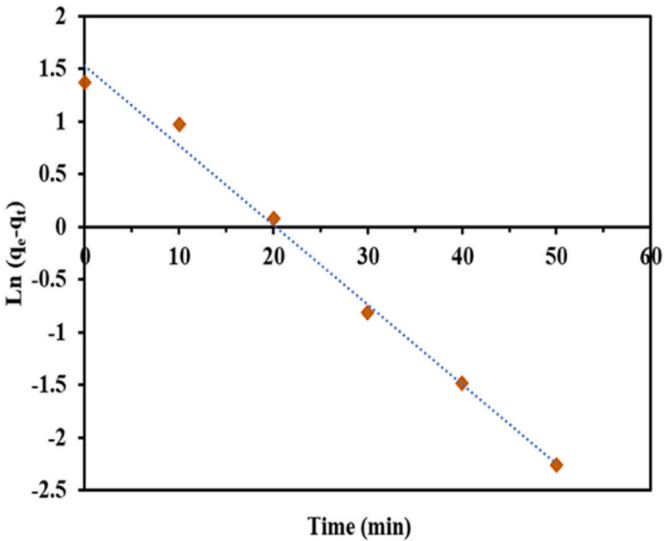
Fig. 12. Pseudo first order kinetic data fits using (pH 3, 20 mg/L and 5 g/L loading).
