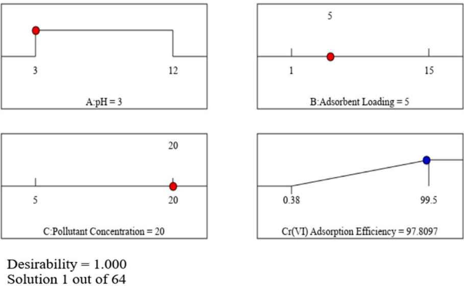
Fig. 10. Ramp plot of numerical optimized conditions with the desirability of 100%.
