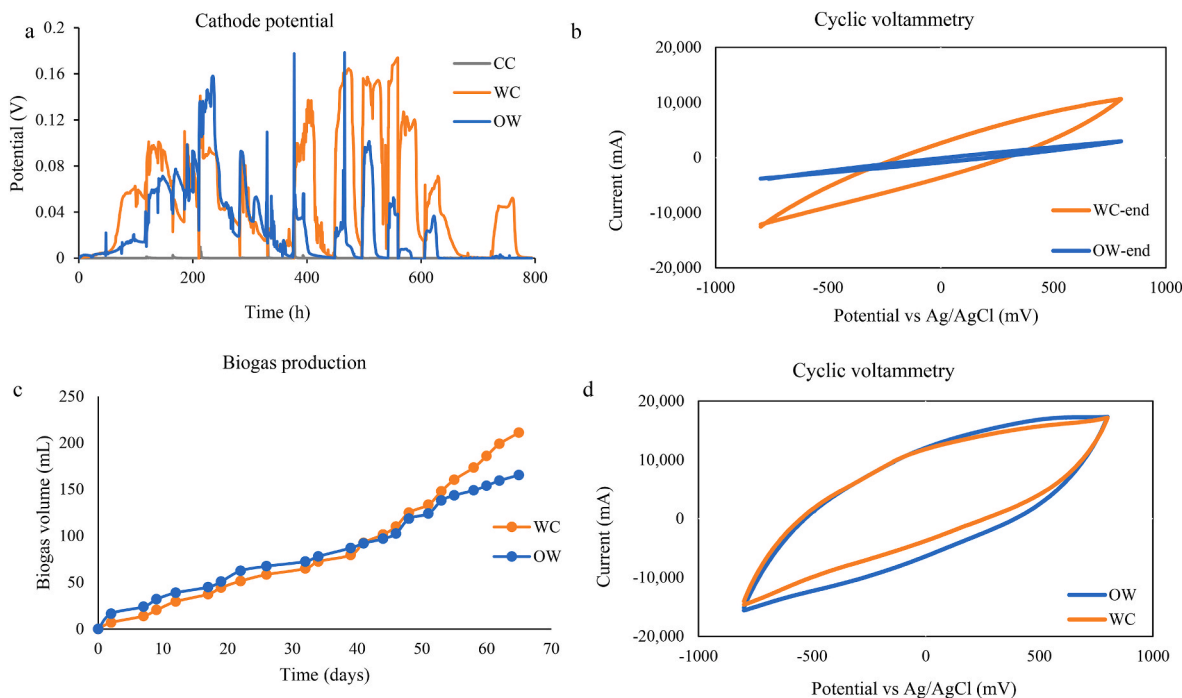
Fig. 1. Cathode potential and cyclic voltammetry of air cathode MFCs and gas volume and cyclic voltammetry in MECs. The CVs were conducted with scan rate of 0.5\text{ mV s}^{-1} in the artificial medium described in 2.2.1 Microbial Fuel Cells. a) Cathode potential of four cycle in MFCs; b) Cyclic voltammograms of woodchip (WC) and organic waste (OW) biochar-based cathodes in MFCs; c) Gas volume in MECs; d) Cyclic voltammograms of woodchip (WC) and organic waste (OW) biochar-based cathodes in MECs.
