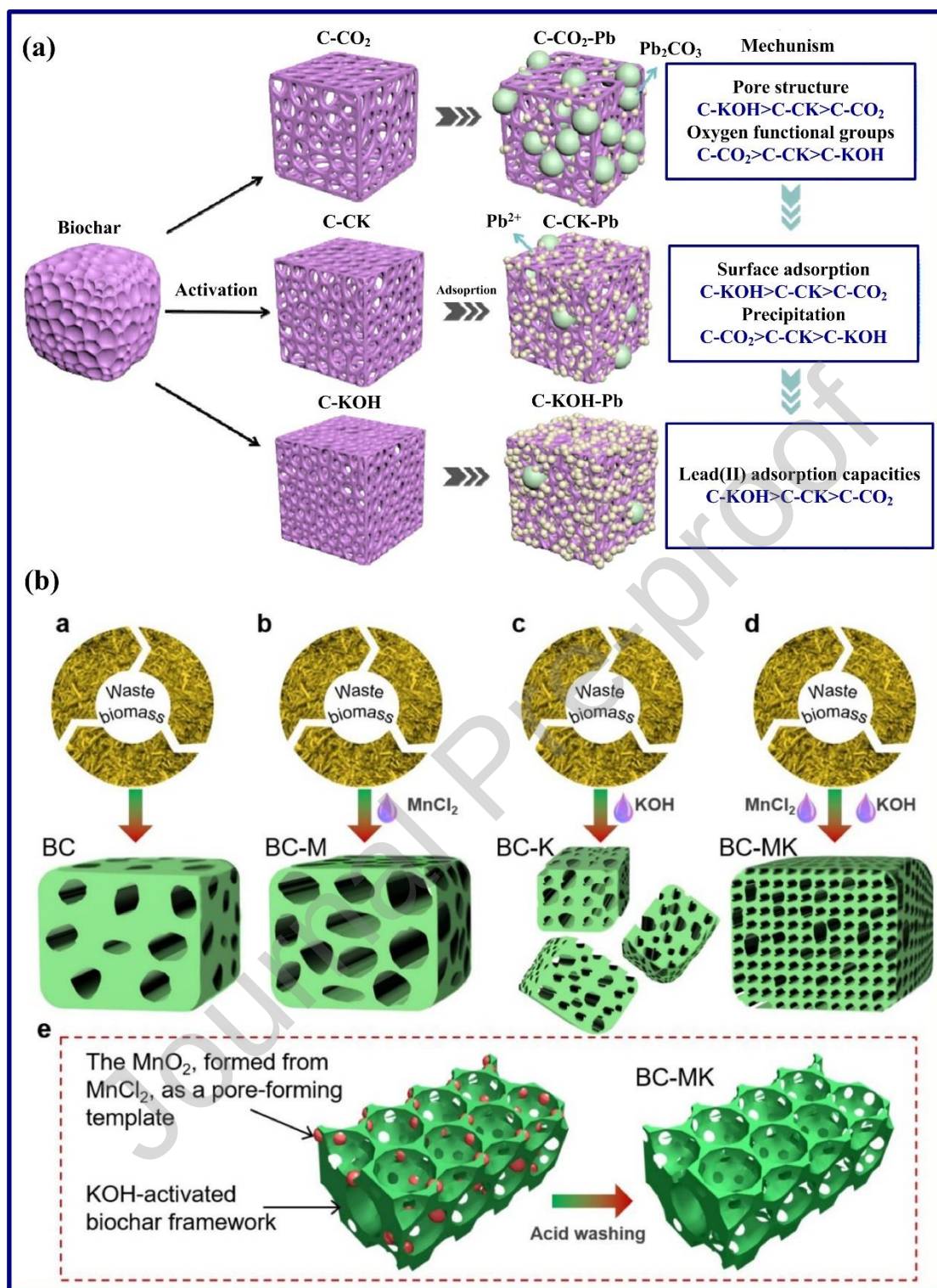
Figure 4. (a) Advantages of KOH chemical activation reported by Zhang et al. [107], reprinted with the permission from Elsevier, Copyright © 2024. License number: 5758451160125, (b) \text{MnCl}_2/\text{KOH} dual chemical activation strategy reported by Zhang et al. [109], reprinted with the permission from Elsevier, Copyright © 2023. License number: 5779121388817
